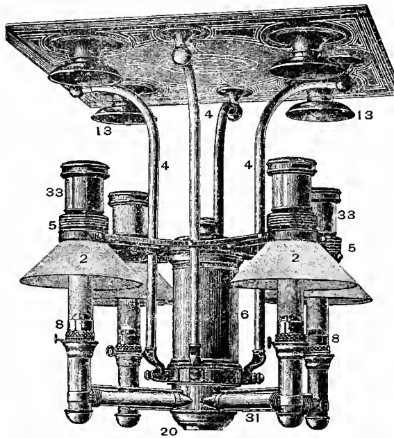
Fig. 3273. For Postal Cars. One Oil Fountain. Mochring's Center-draft Burner. Drop, 30 ins.
